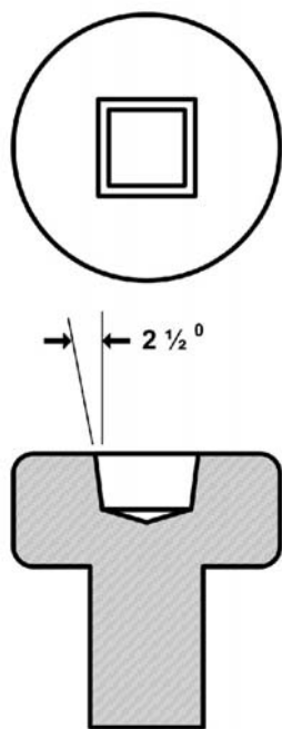
Square Socket Recess ASME Type III
